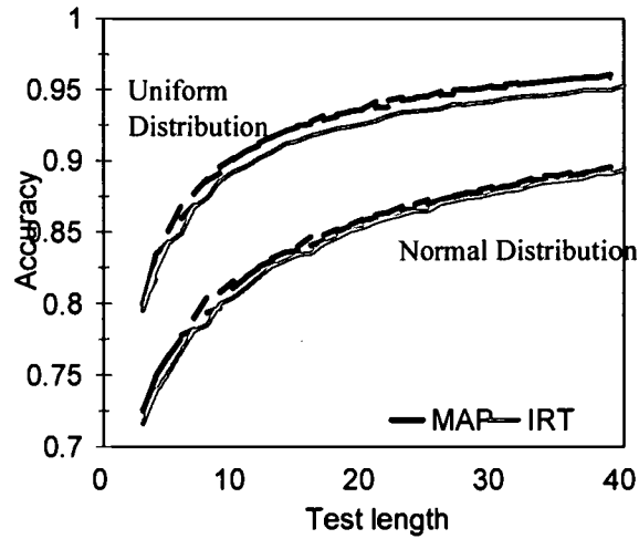
Figure 1: Accuracy of decision theory (MAP), and IRT scoring as a function of test length and ability distribution for simulated tests based on CSAP.
